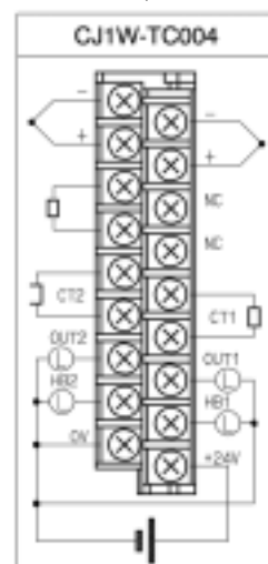
CJ1W-TC004 (2 loop, allarme HB, uscite PNP)
