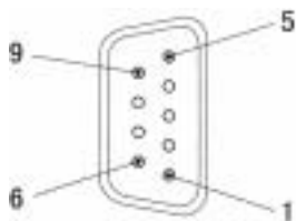
Porta RS422/485
